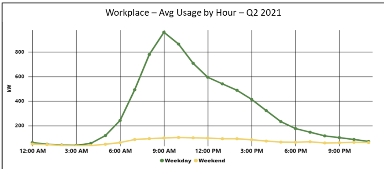
Figure 4.1 Workplace Average Usage per Hour in Q1 2021: 64 sites/1474 ports
