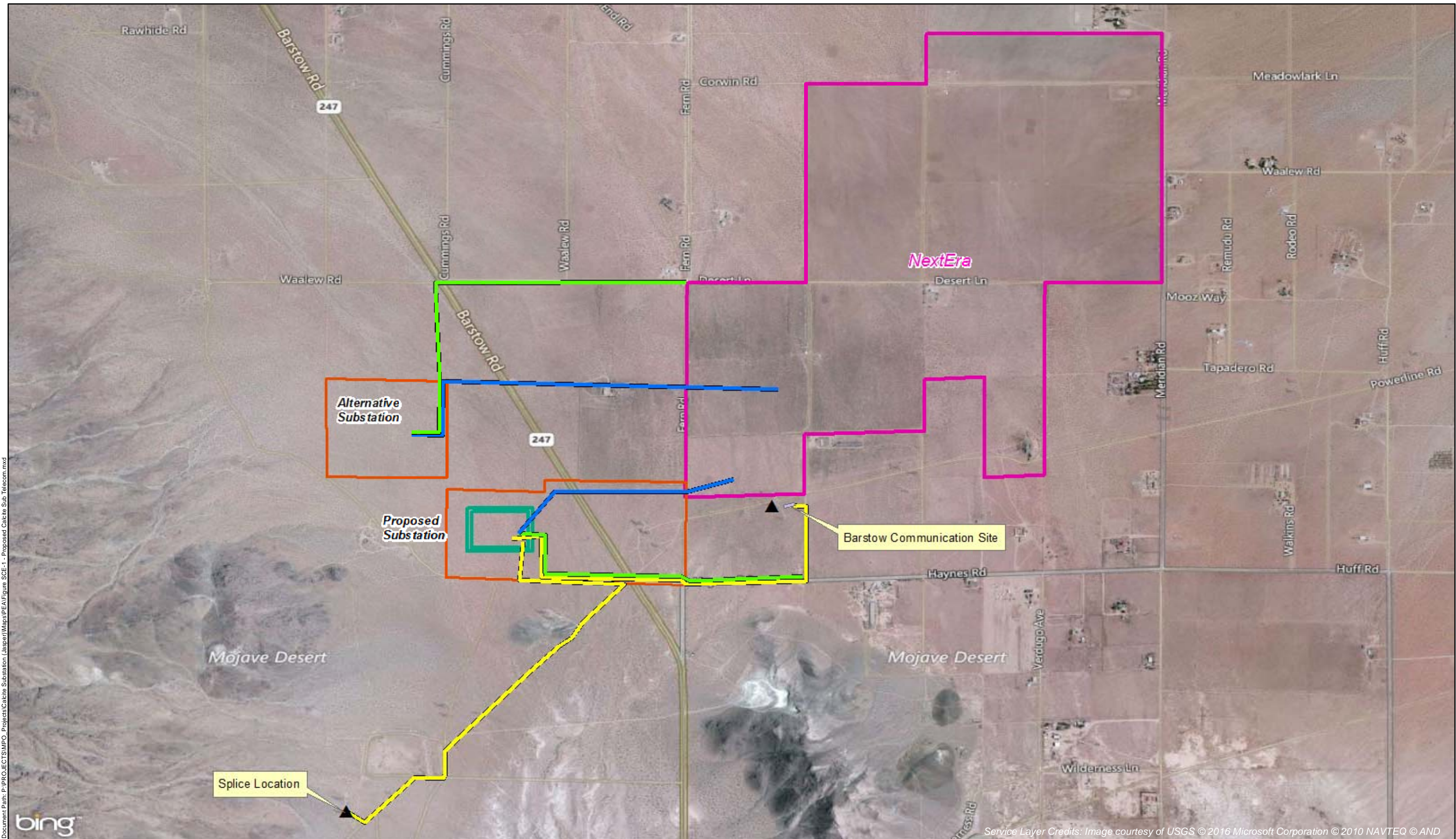
FIGURE SCE-1 PROPOSED AND ALTERNATIVE CALCITE SUBSTATION, DISTRIBUTION AND TELECOMMUNICATION LINES
